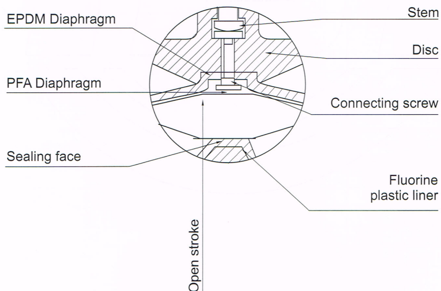
(2) Sealing principle
