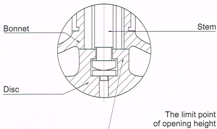
(1) Limit principle
